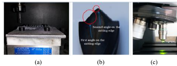
Fig. 3. (a) Experimental setup; (b) drill bit used in the experiments; (c) edge radius measurement.
